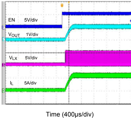
Startup from Enable ( V_{IN}=5.0V, V_{OUT}=1.0V, I_O=6.0A )
