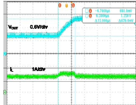
Dynamic Voltage Switch [ V_{IN}=6.0V , 0A Load, V_{OUT}=0.7125\sim 1.5V , Slow Rate= 12.6mV/19.2\mu s ]
