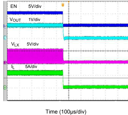
Shutdown from Enable ( V_{IN}=5.0V, V_{OUT}=1.0V, I_O=6.0A )
