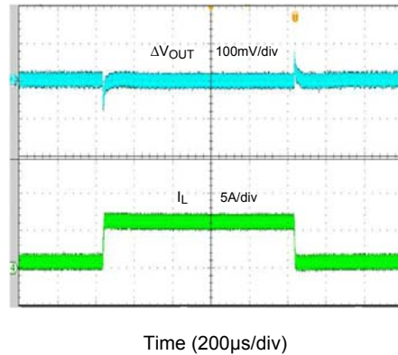
Load Transient ( V_{IN}=5.0V, V_{OUT}=1.0V, I_O=0.6 \sim 6.0A )
